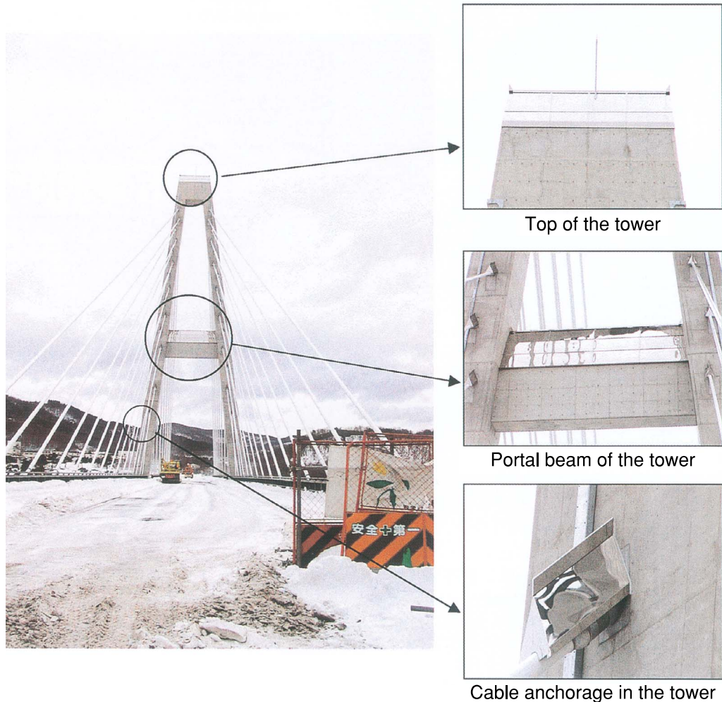
Photo. 5 The example of application of titanium panel for snow sliding to HOSHINOFURUSATO BRIDGE (Ashibetsu, Hokkaido). 星の降る里大橋 (芦別市)
